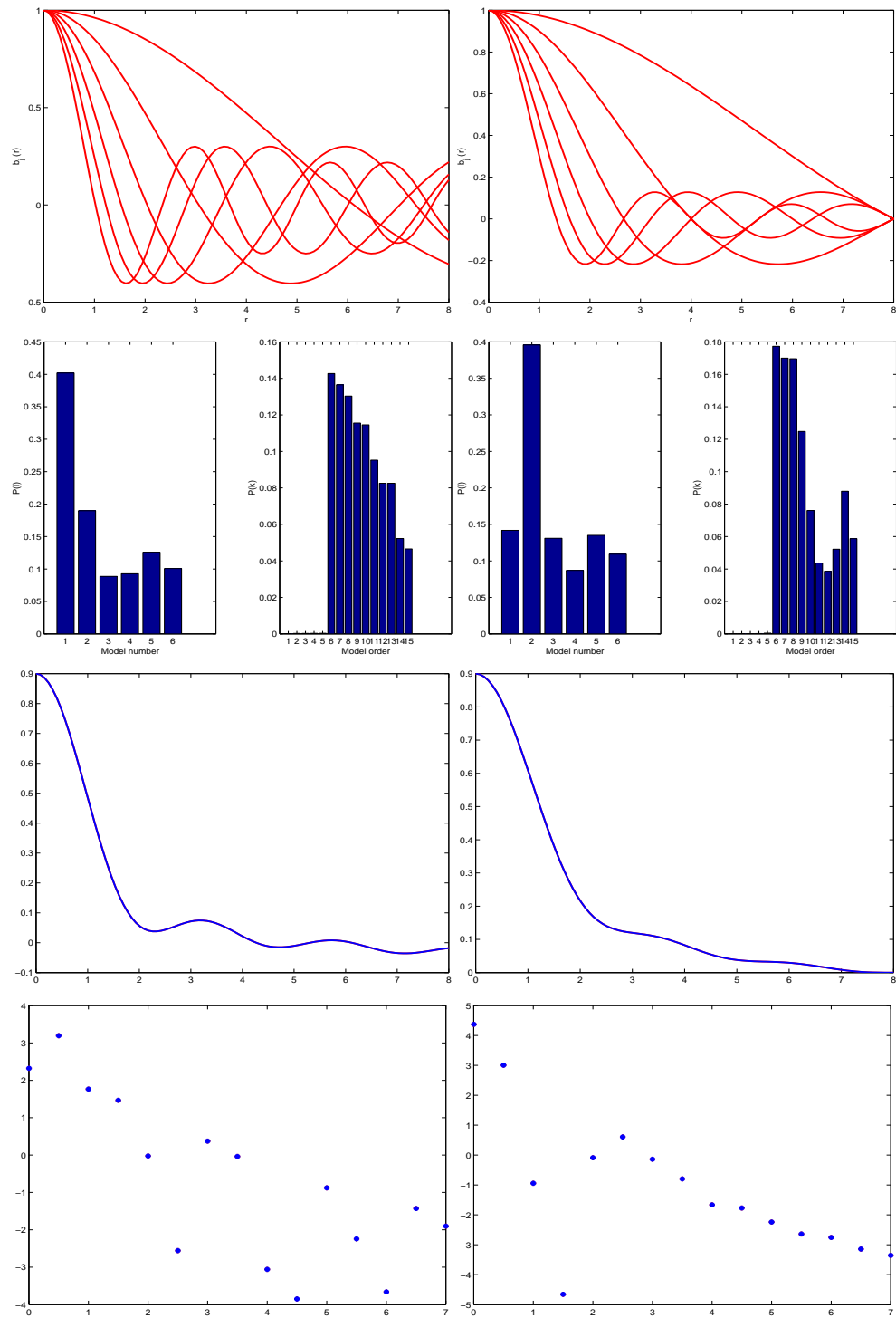
Fig. 3: Left: l = 1 Right: l = 2 a) basis functions b_j(r) , b) p(k|\mathbf{y}) and p(k|\mathbf{y}, \hat{l}) , c) \rho(r) and \hat{\rho}(r) , d) F(q_i) and \hat{F}(q_i) .
